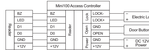
Figure 2 : Wiring Diagram
