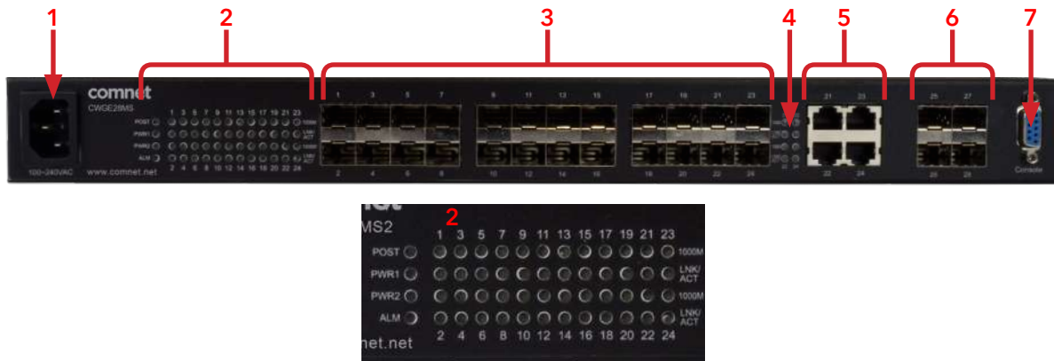
CWGE28MS Front Panel
