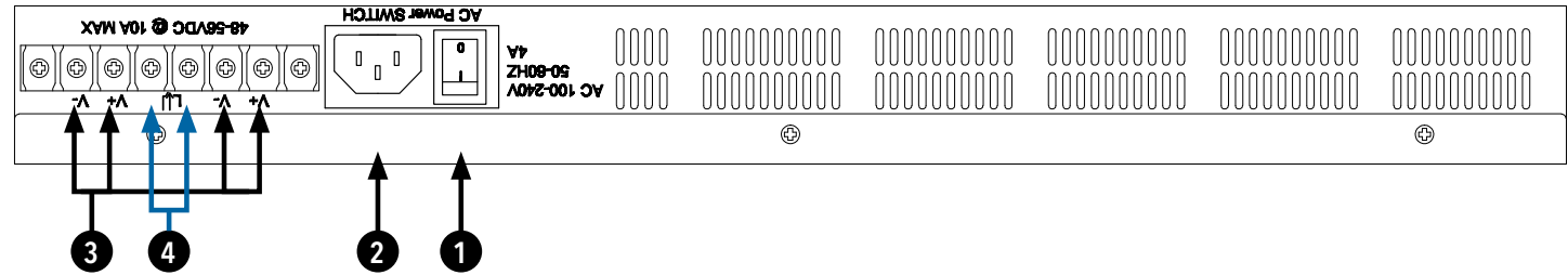
CNGE24FX12TX12MS[POE] Rear Panel
